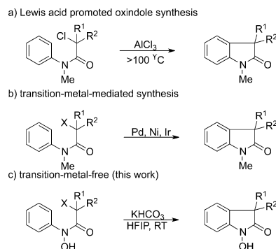
Scheme 1. Access to oxindoles from \alpha -halo anilides.
