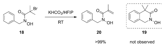
Scheme 5. Control experiment.
